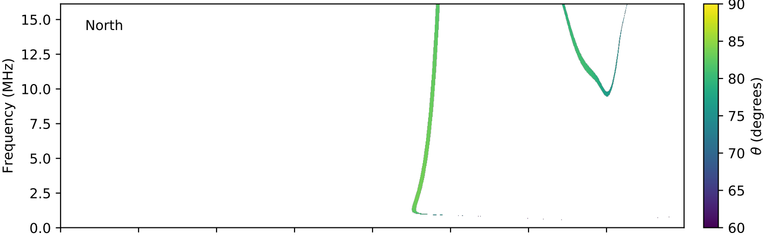
expres_cassini_jupiter_europa_isaac_lossc-wid1deg_3kev_20021129_v01.cdf
