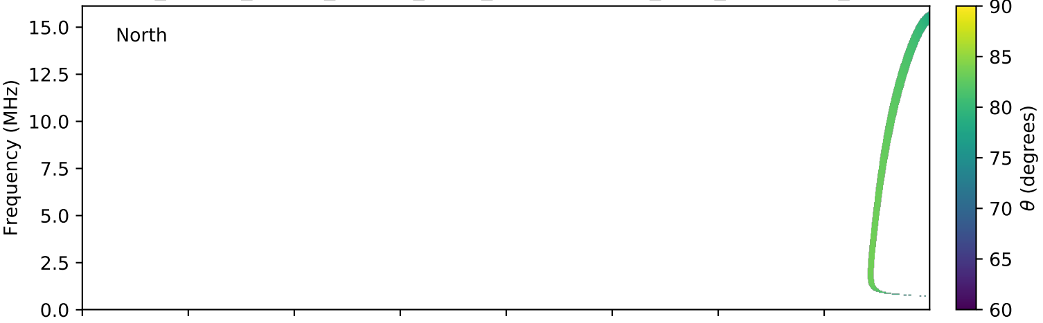
expres_cassini_jupiter_europa_isaac_lossc-wid1deg_3kev_20021125_v01.cdf
