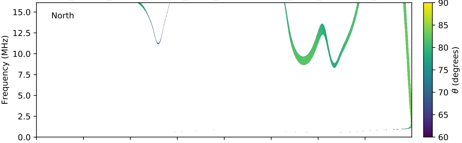
expres_cassini_jupiter_europa_isaac_lossc-wid1deg_3kev_20021123_v01.cdf
