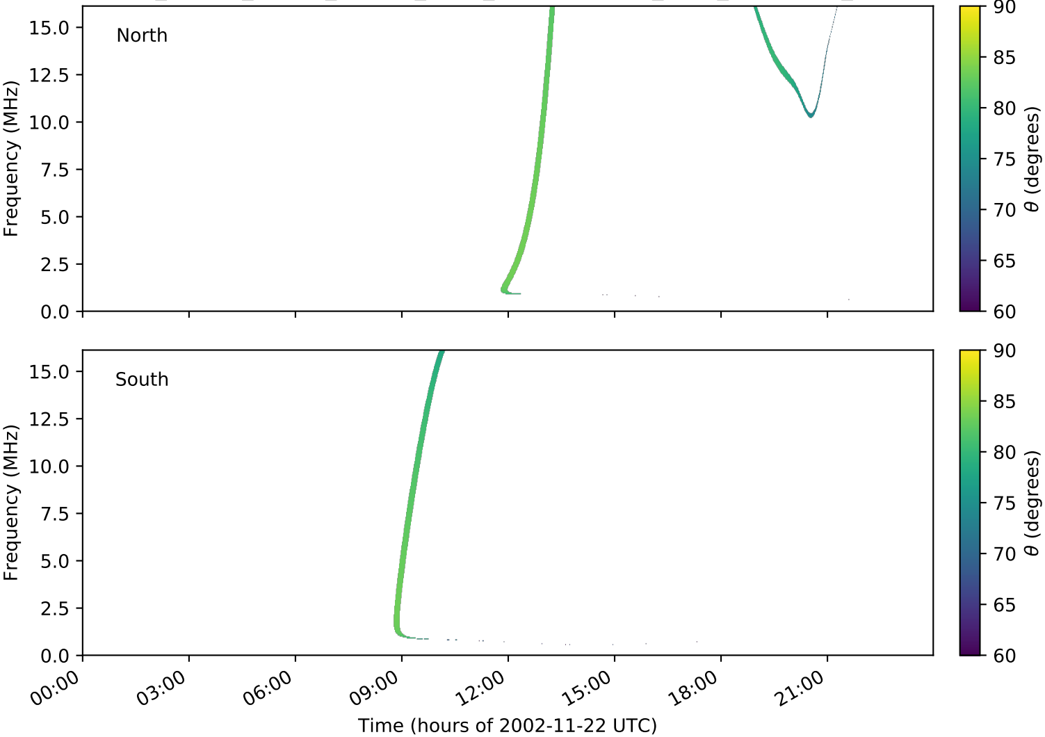
expres_cassini_jupiter_europa_isaac_lossc-wid1deg_3kev_20021122_v01.cdf
