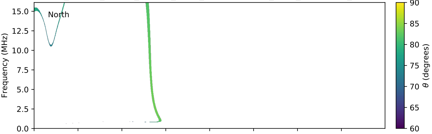
expres_cassini_jupiter_europa_isaac_lossc-wid1deg_3kev_20021120_v01.cdf
