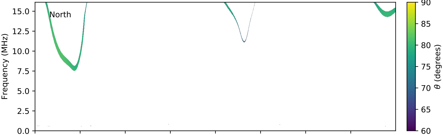
expres_cassini_jupiter_europa_isaac_lossc-wid1deg_3kev_20021119_v01.cdf
