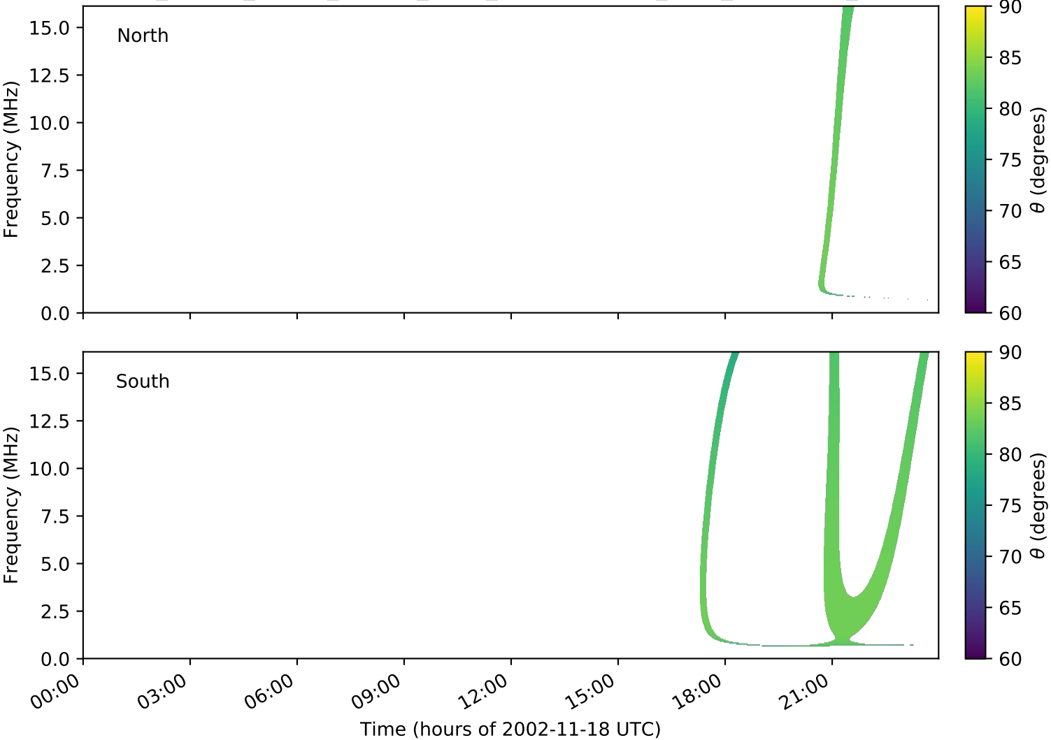
expres_cassini_jupiter_europa_isaac_lossc-wid1deg_3kev_20021118_v01.cdf
