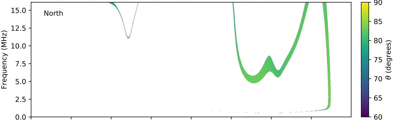
expres_cassini_jupiter_europa_isaac_lossc-wid1deg_3kev_20021116_v01.cdf
