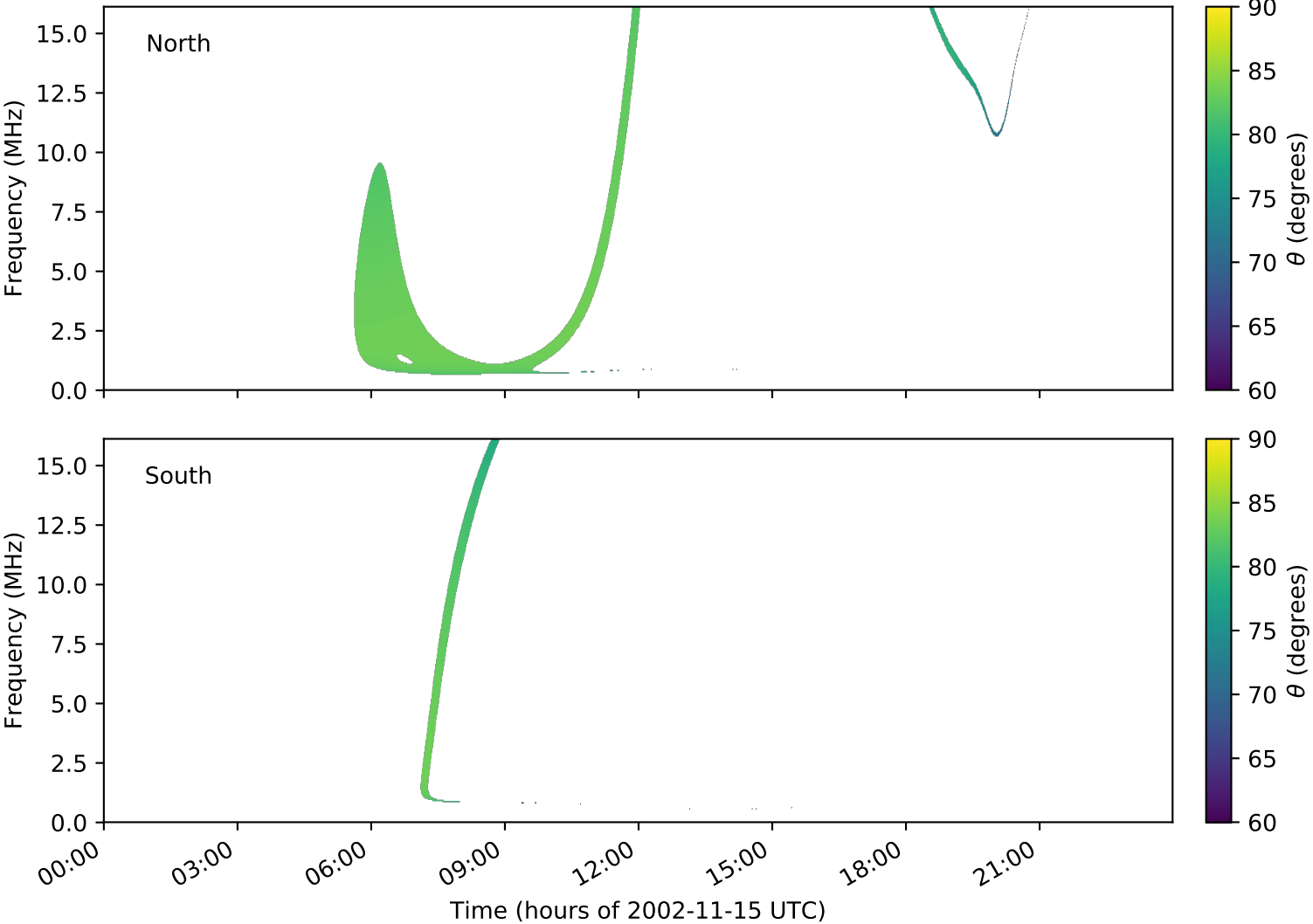
expres_cassini_jupiter_europa_isaac_lossc-wid1deg_3kev_20021115_v01.cdf
