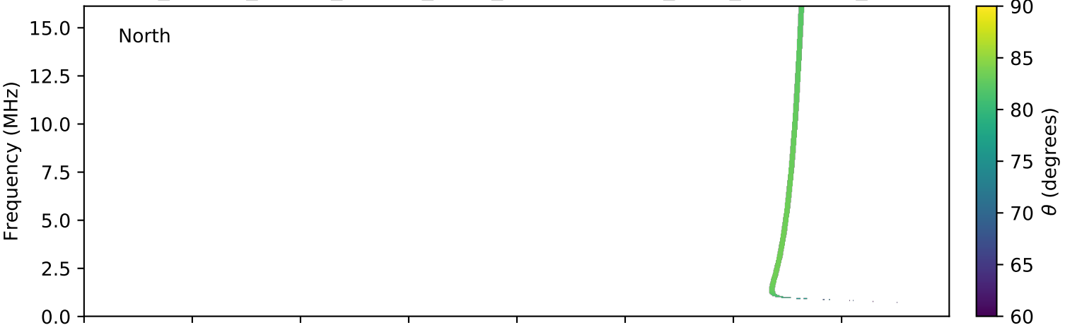
expres_cassini_jupiter_europa_isaac_lossc-wid1deg_3kev_20021111_v01.cdf
