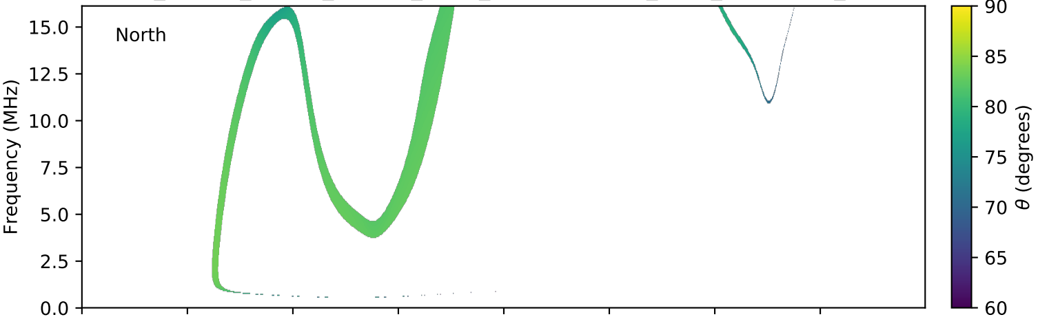
expres_cassini_jupiter_europa_isaac_lossc-wid1deg_3kev_20021108_v01.cdf
