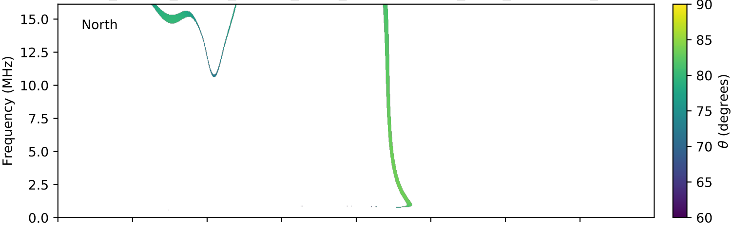
expres_cassini_jupiter_europa_isaac_lossc-wid1deg_3kev_20021102_v01.cdf
