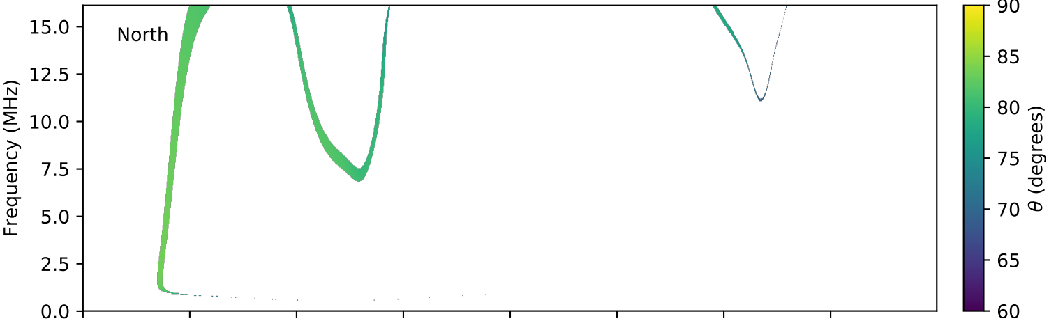
expres_cassini_jupiter_europa_isaac_lossc-wid1deg_3kev_20021101_v01.cdf
