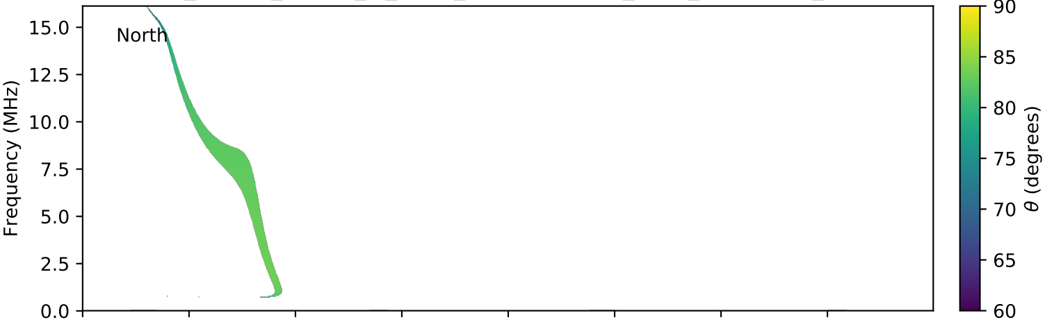
expres_cassini_jupiter_io_isaac_lossc-wid1deg_3kev_20021031_v01.cdf
