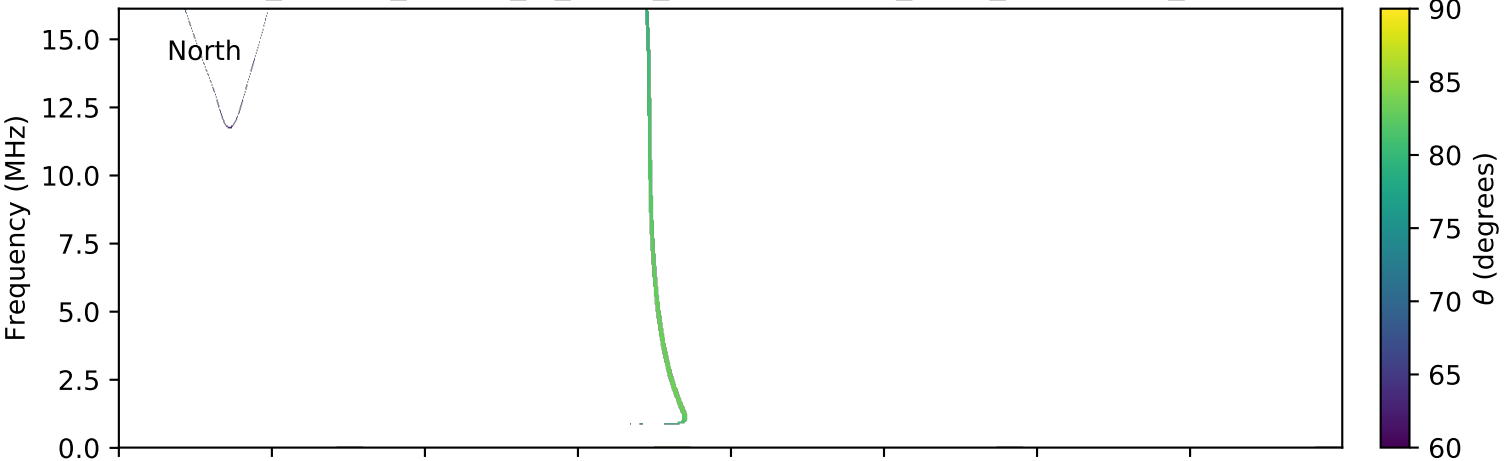
expres_cassini_jupiter_io_isaac_lossc-wid1deg_3kev_20021029_v01.cdf
