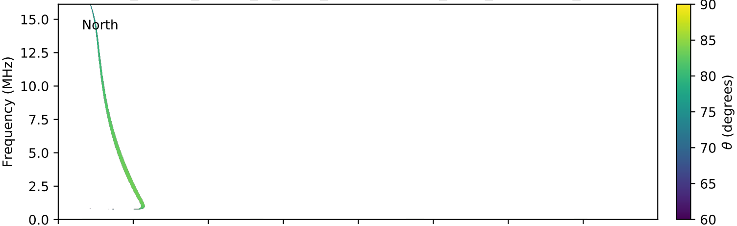
expres_cassini_jupiter_io_isaac_lossc-wid1deg_3kev_20021024_v01.cdf
