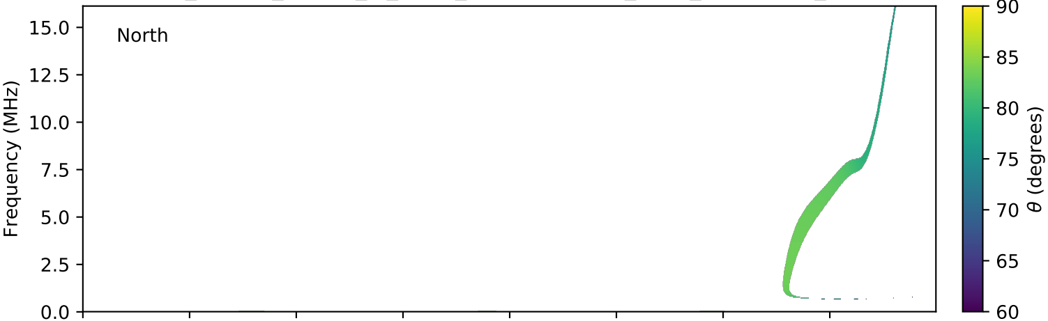
expres_cassini_jupiter_io_isaac_lossc-wid1deg_3kev_20021019_v01.cdf
