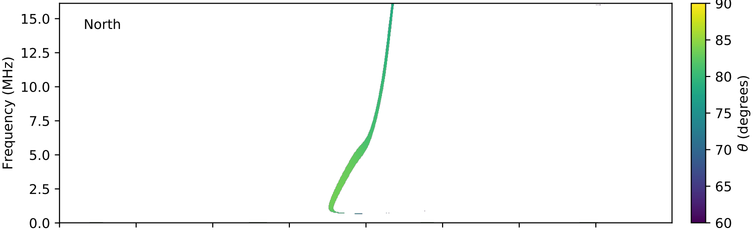
expres_cassini_jupiter_io_isaac_lossc-wid1deg_3kev_20021007_v01.cdf
