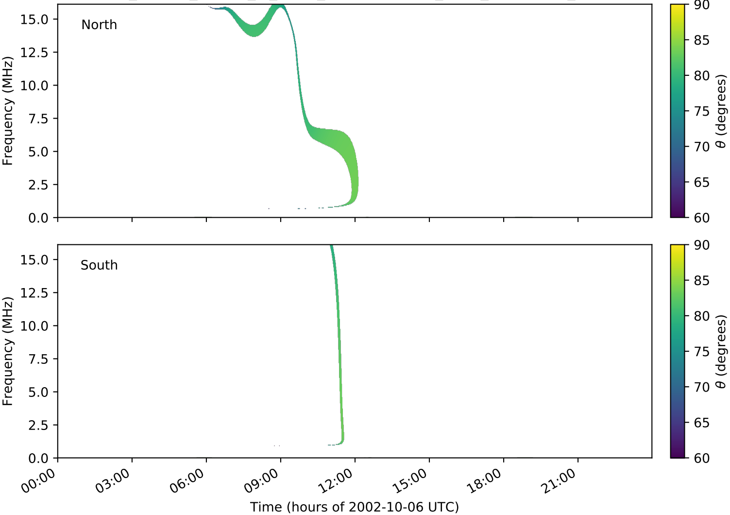
expres_cassini_jupiter_io_isaac_lossc-wid1deg_3kev_20021006_v01.cdf
