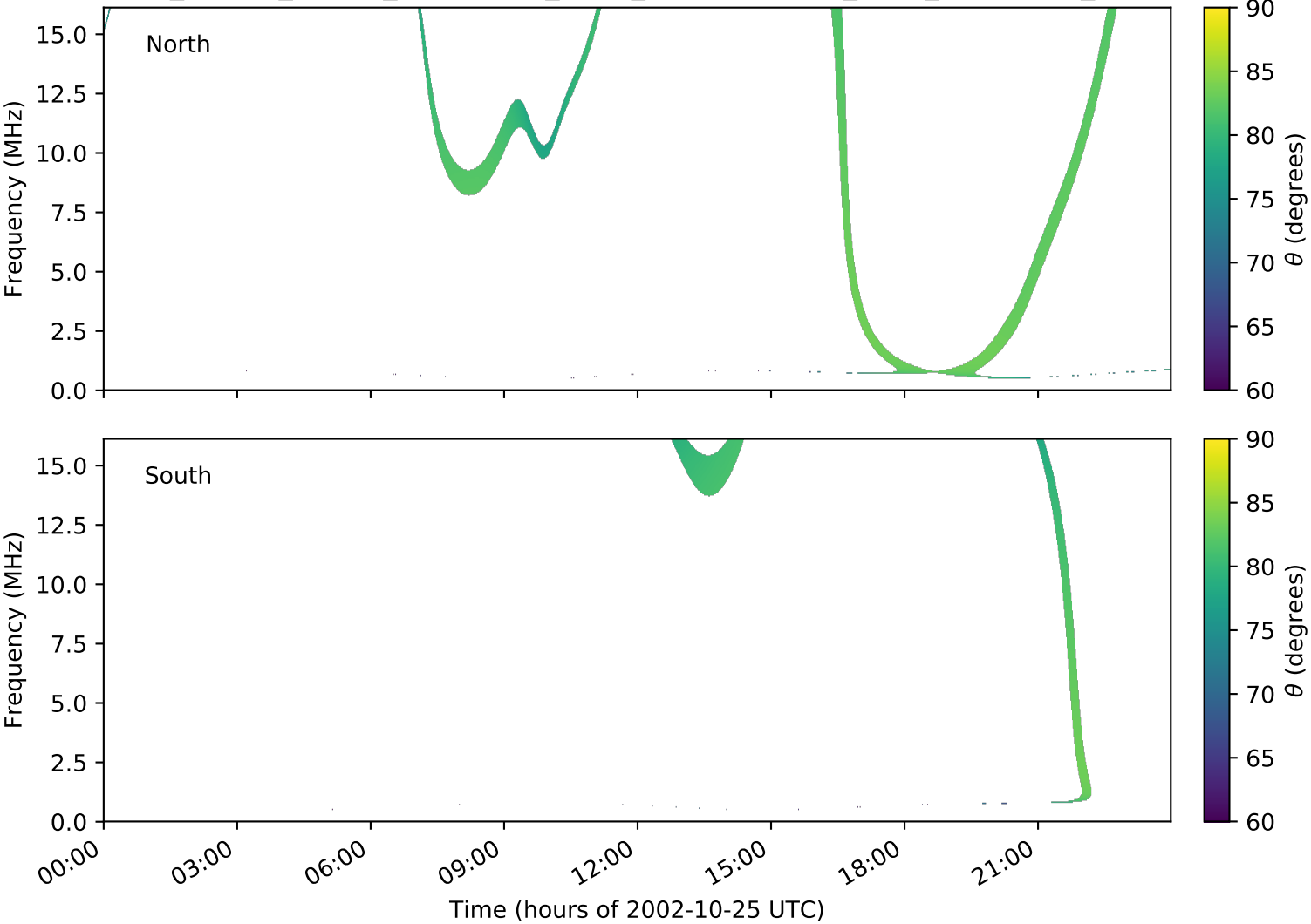
expres_cassini_jupiter_ganymede_isaac_lossc-wid1deg_3kev_20021025_v01.cdf
