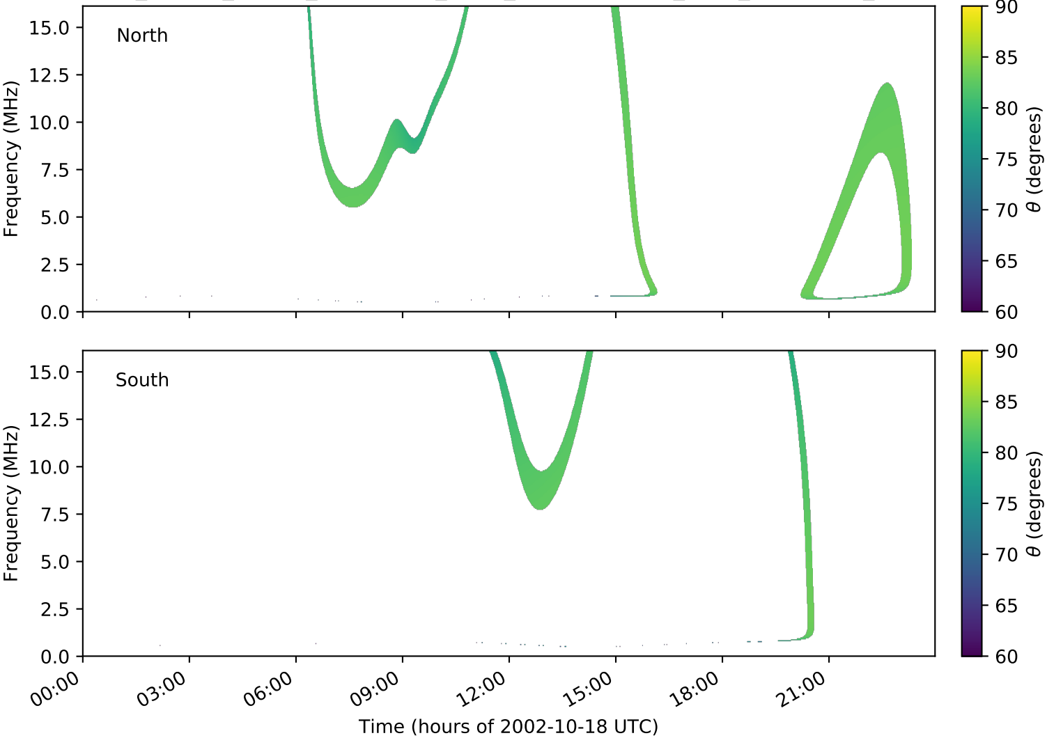
expres_cassini_jupiter_ganymede_isaac_lossc-wid1deg_3kev_20021018_v01.cdf
