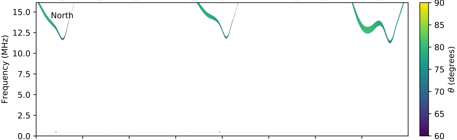
expres_cassini_jupiter_ganymede_isaac_lossc-wid1deg_3kev_20021017_v01.cdf
