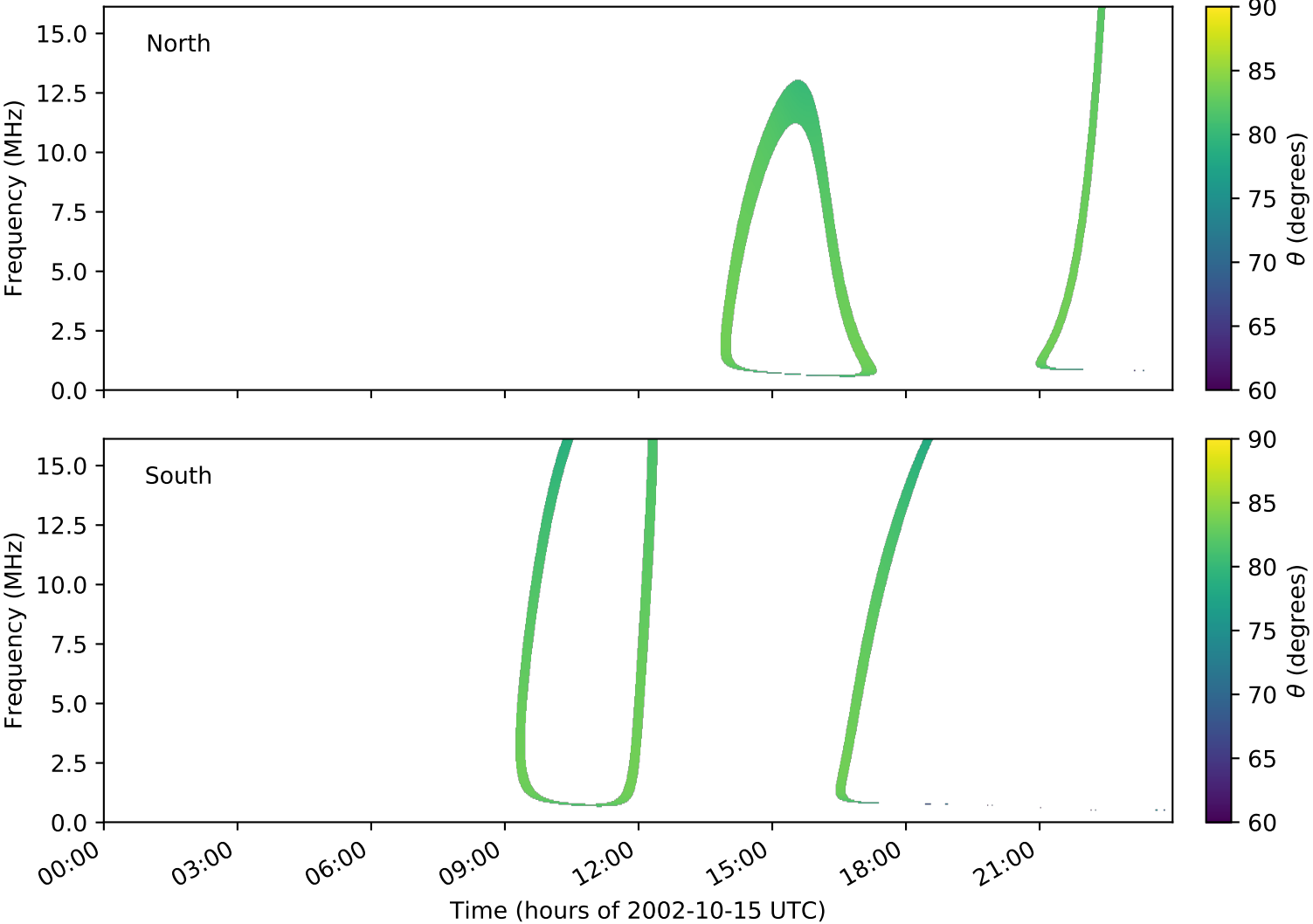
expres_cassini_jupiter_ganymede_isaac_lossc-wid1deg_3kev_20021015_v01.cdf
