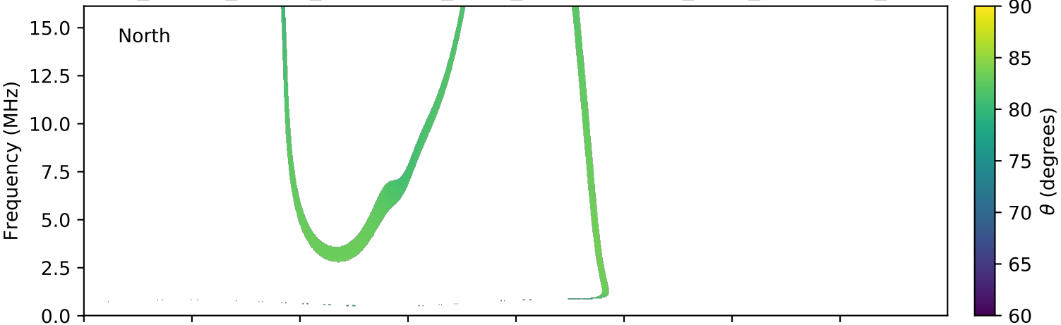
expres_cassini_jupiter_ganymede_isaac_lossc-wid1deg_3kev_20021011_v01.cdf
