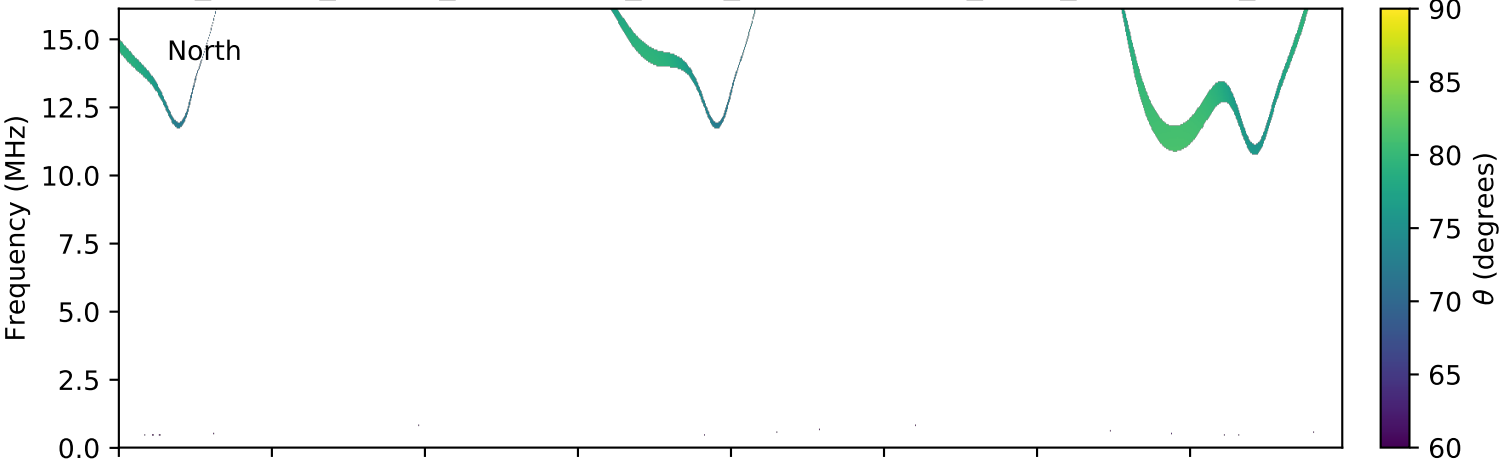
expres_cassini_jupiter_ganymede_isaac_lossc-wid1deg_3kev_20021010_v01.cdf
