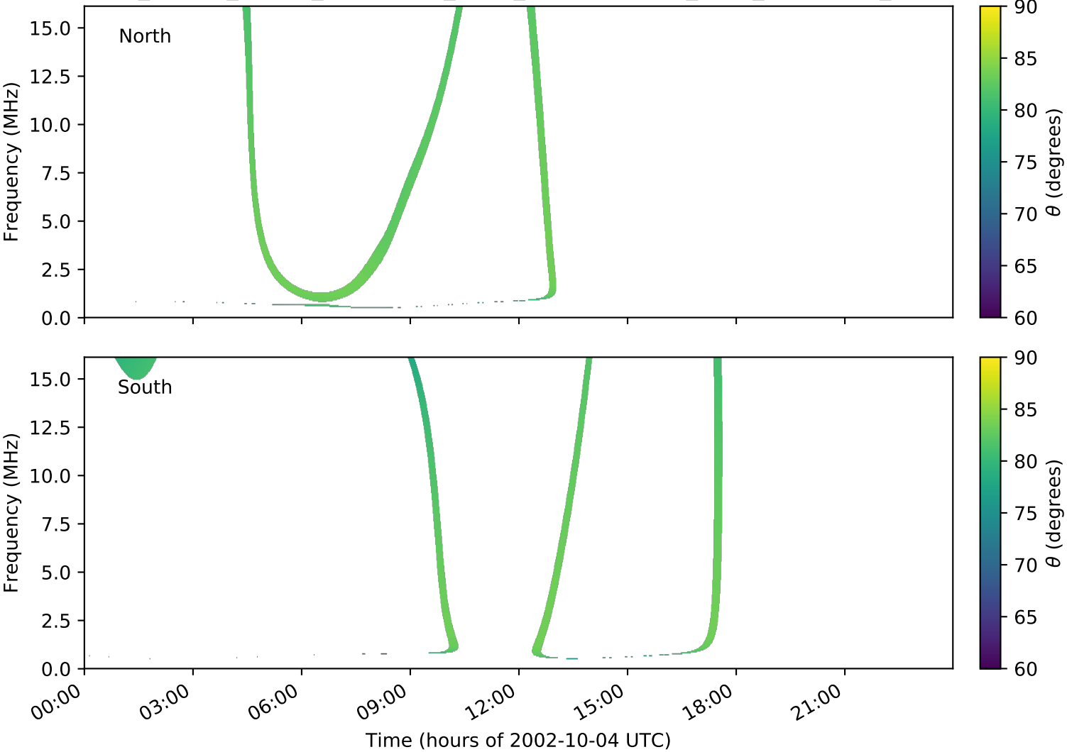
expres_cassini_jupiter_ganymede_isaac_lossc-wid1deg_3kev_20021004_v01.cdf
