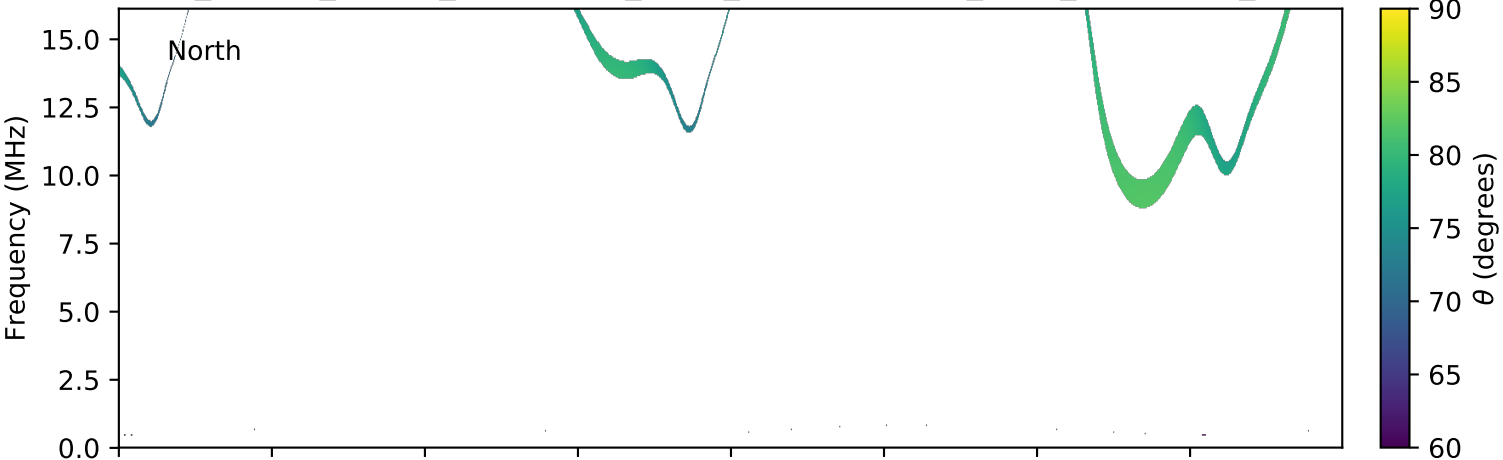
expres_cassini_jupiter_ganymede_isaac_lossc-wid1deg_3kev_20021003_v01.cdf
