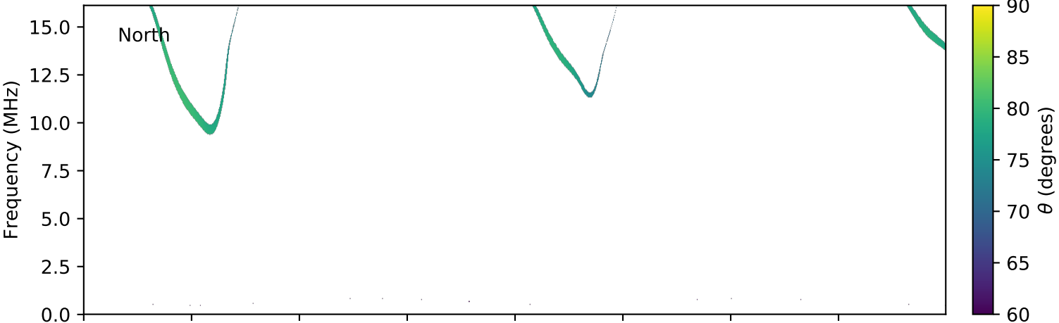
expres_cassini_jupiter_ganymede_isaac_lossc-wid1deg_3kev_20021002_v01.cdf
