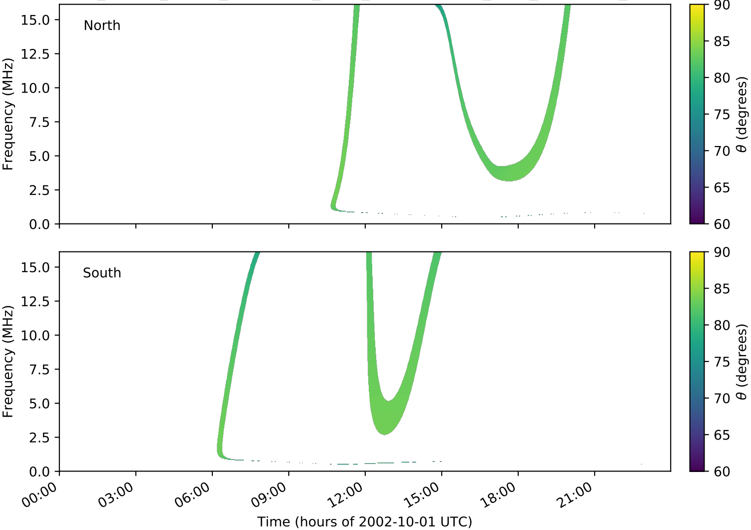
expres_cassini_jupiter_ganymede_isaac_lossc-wid1deg_3kev_20021001_v01.cdf
