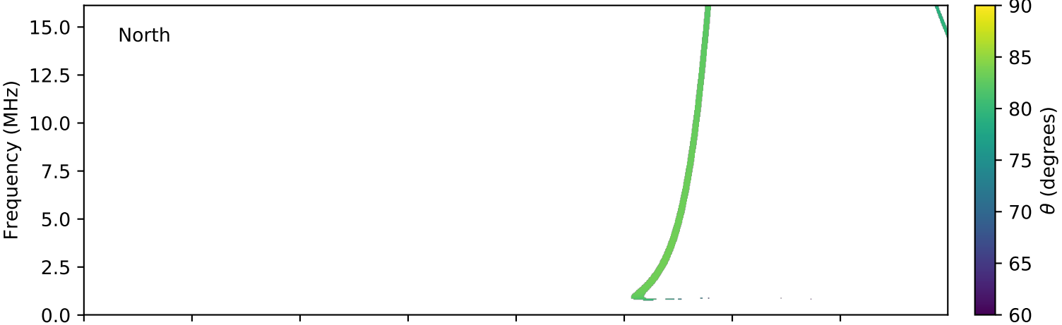
expres_cassini_jupiter_europa_isaac_lossc-wid1deg_3kev_20021028_v01.cdf
