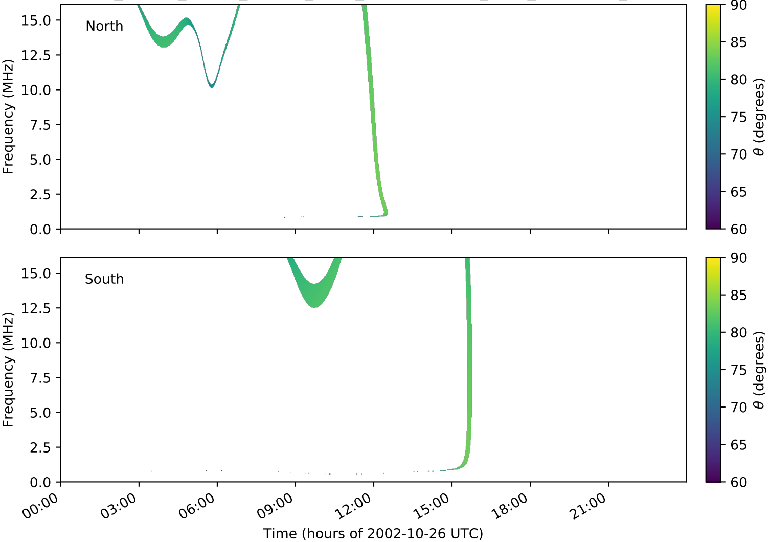
expres_cassini_jupiter_europa_isaac_lossc-wid1deg_3kev_20021026_v01.cdf
