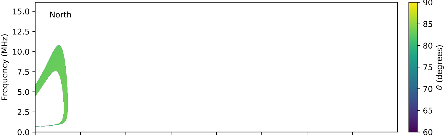
expres_cassini_jupiter_europa_isaac_lossc-wid1deg_3kev_20021023_v01.cdf
