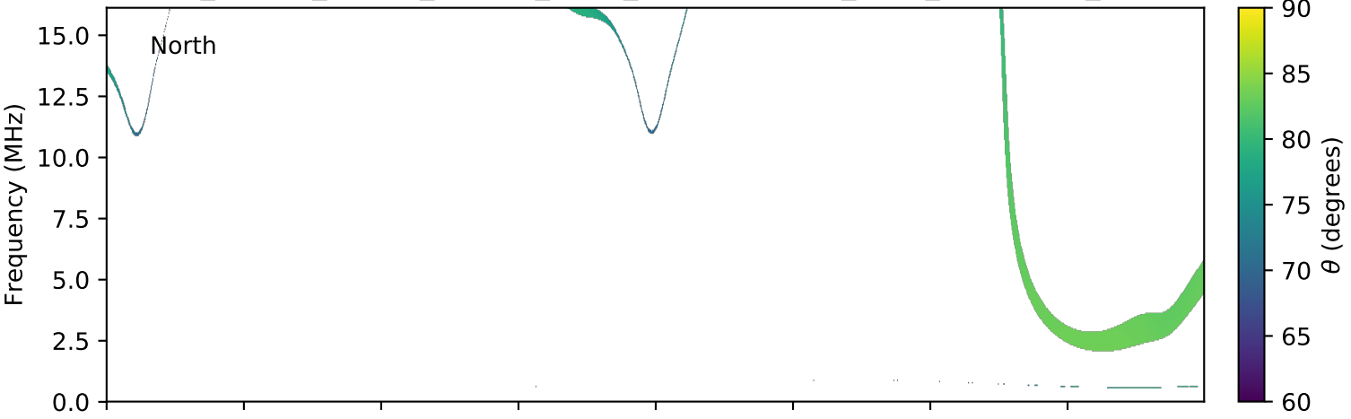
expres_cassini_jupiter_europa_isaac_lossc-wid1deg_3kev_20021022_v01.cdf
