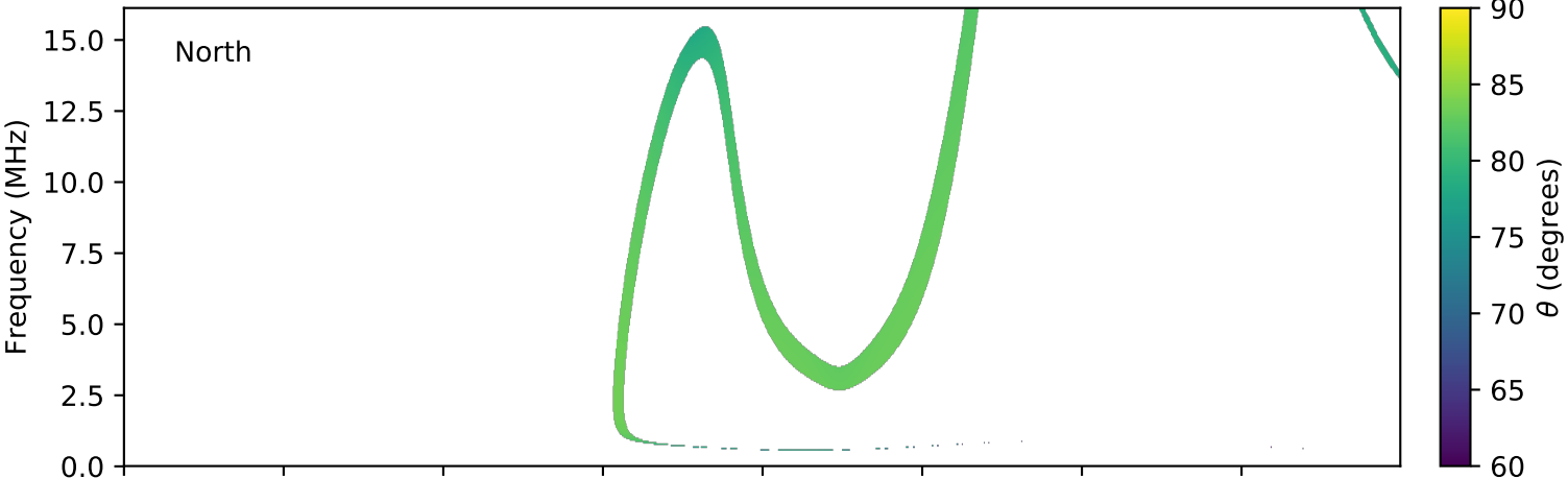
expres_cassini_jupiter_europa_isaac_lossc-wid1deg_3kev_20021021_v01.cdf
