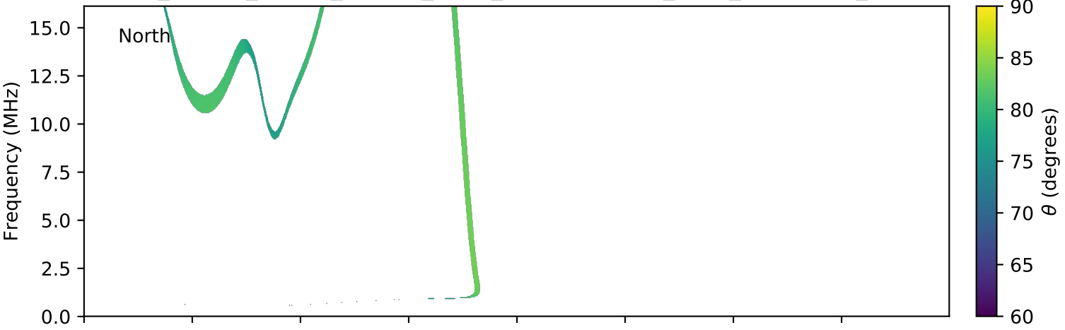
expres_cassini_jupiter_europa_isaac_lossc-wid1deg_3kev_20021019_v01.cdf
