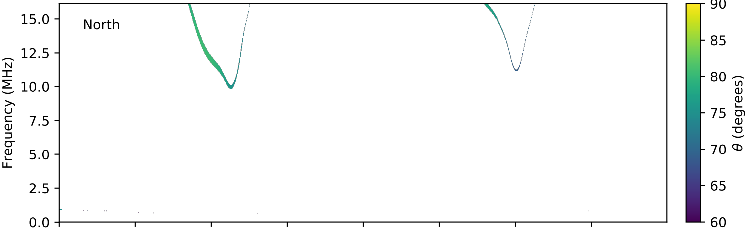
expres_cassini_jupiter_europa_isaac_lossc-wid1deg_3kev_20021018_v01.cdf
