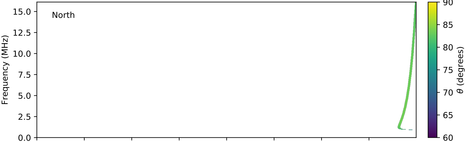
expres_cassini_jupiter_europa_isaac_lossc-wid1deg_3kev_20021017_v01.cdf
