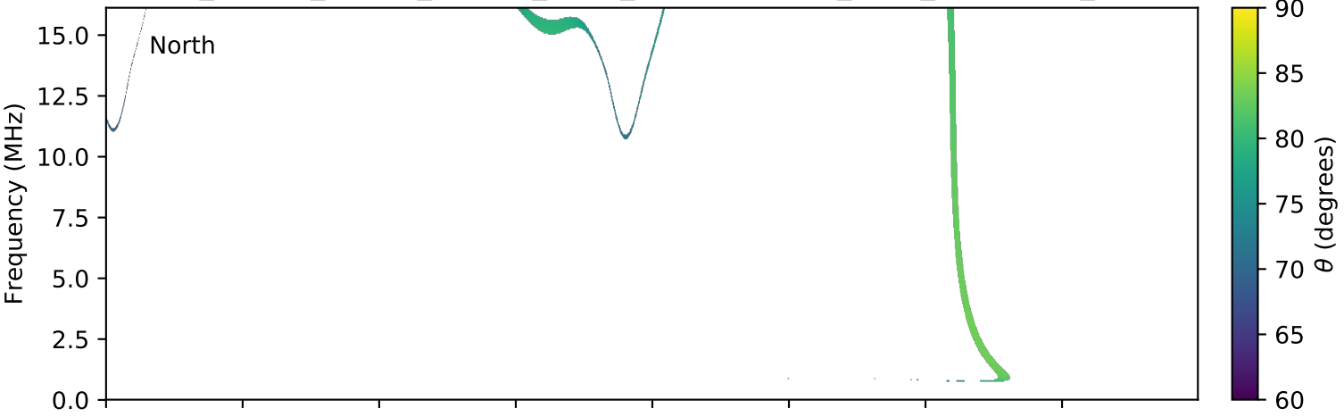
expres_cassini_jupiter_europa_isaac_lossc-wid1deg_3kev_20021015_v01.cdf
