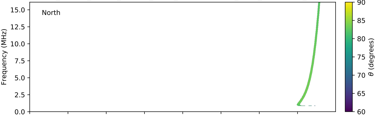
expres_cassini_jupiter_europa_isaac_lossc-wid1deg_3kev_20021010_v01.cdf
