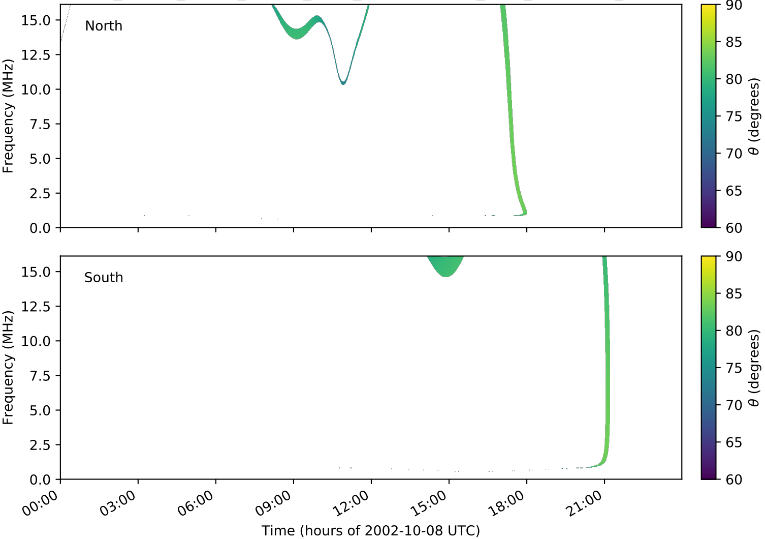
expres_cassini_jupiter_europa_isaac_lossc-wid1deg_3kev_20021008_v01.cdf
