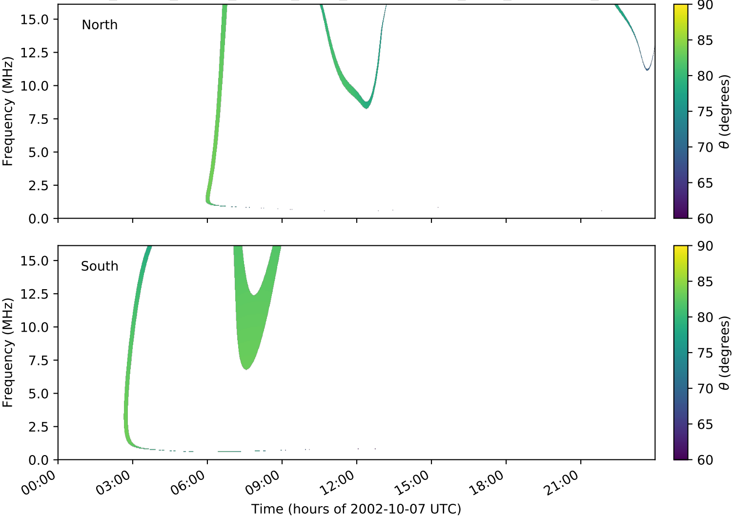
expres_cassini_jupiter_europa_isaac_lossc-wid1deg_3kev_20021007_v01.cdf
