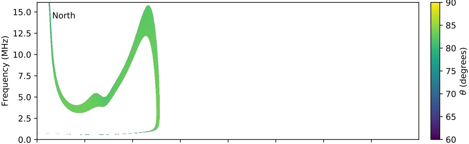
expres_cassini_jupiter_europa_isaac_lossc-wid1deg_3kev_20021005_v01.cdf
