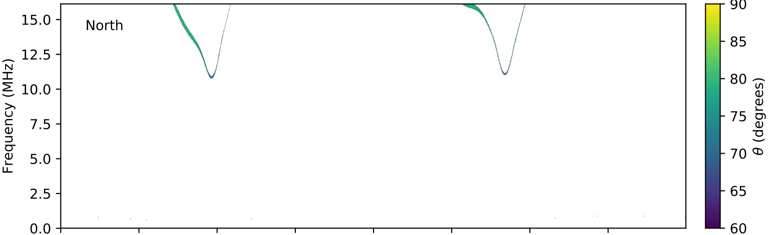
expres_cassini_jupiter_europa_isaac_lossc-wid1deg_3kev_20021004_v01.cdf
