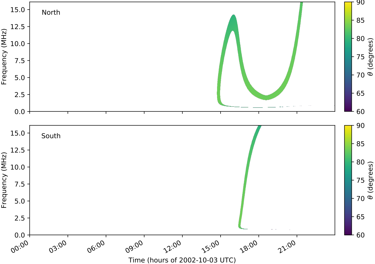
expres_cassini_jupiter_europa_isaac_lossc-wid1deg_3kev_20021003_v01.cdf
