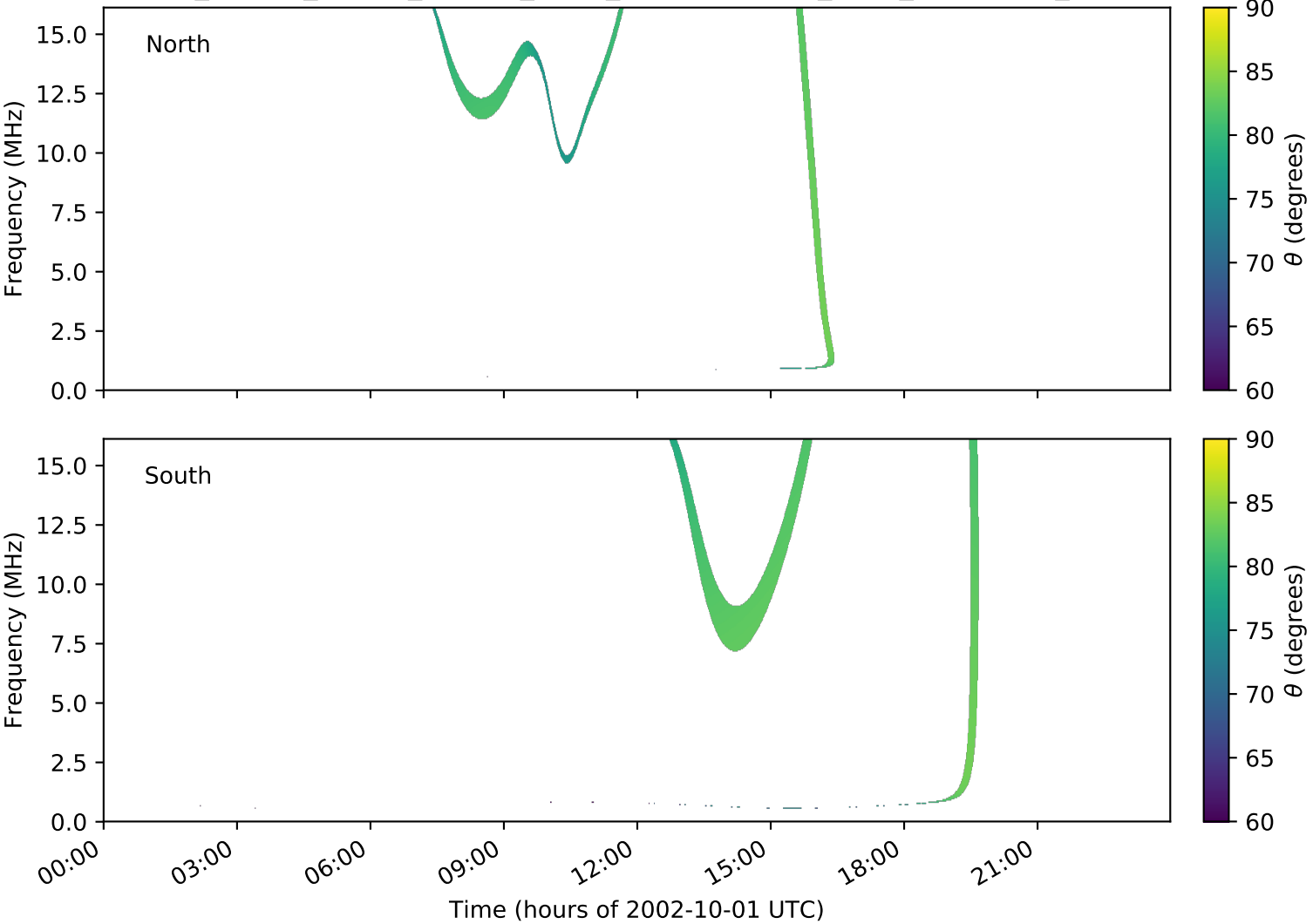
expres_cassini_jupiter_europa_isaac_lossc-wid1deg_3kev_20021001_v01.cdf
