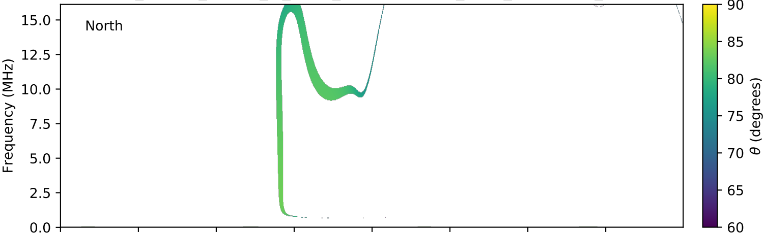
expres_cassini_jupiter_io_isaac_lossc-wid1deg_3kev_20020930_v01.cdf
