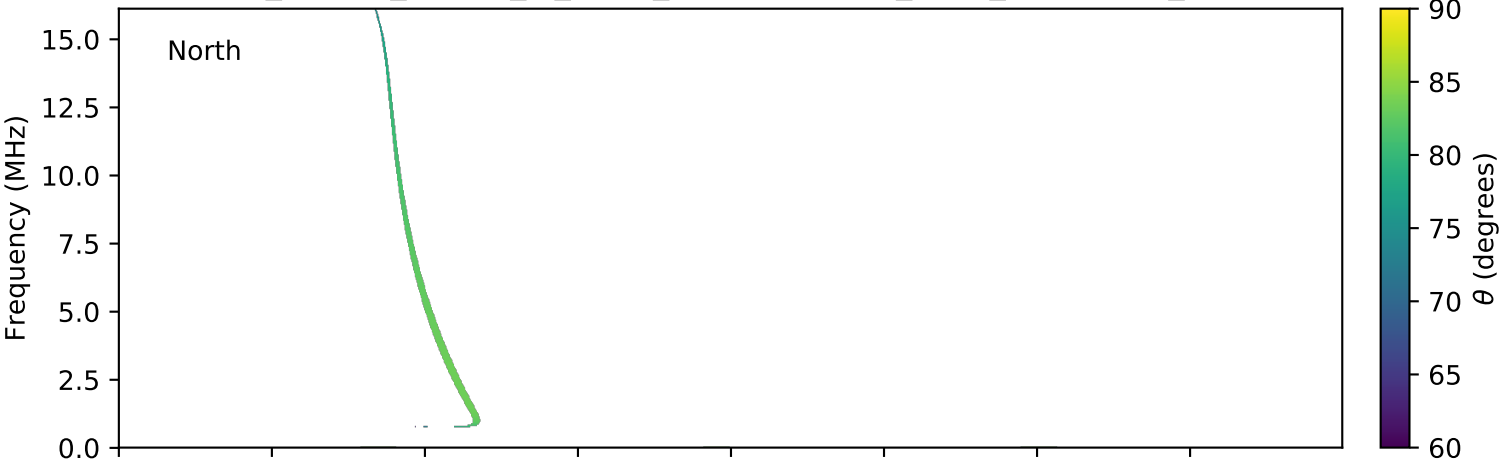
expres_cassini_jupiter_io_isaac_lossc-wid1deg_3kev_20020922_v01.cdf
