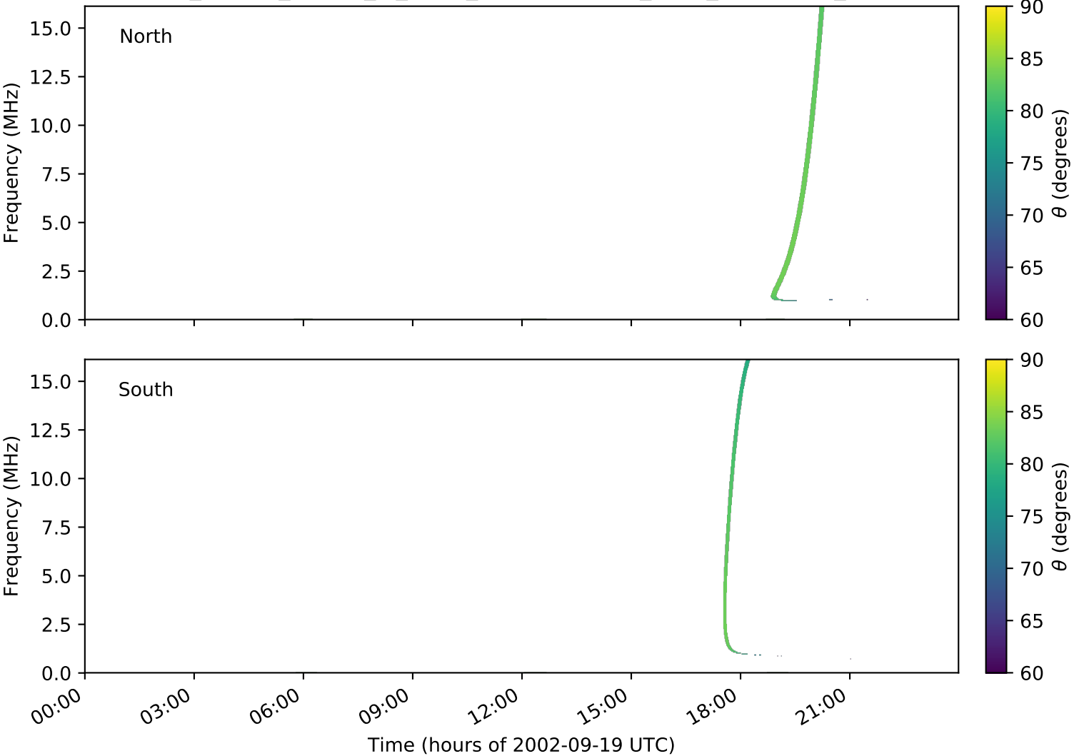
expres_cassini_jupiter_io_isaac_lossc-wid1deg_3kev_20020919_v01.cdf
