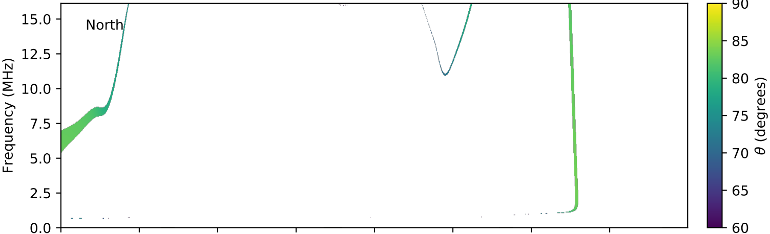
expres_cassini_jupiter_io_isaac_lossc-wid1deg_3kev_20020918_v01.cdf
