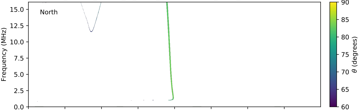
expres_cassini_jupiter_io_isaac_lossc-wid1deg_3kev_20020913_v01.cdf
